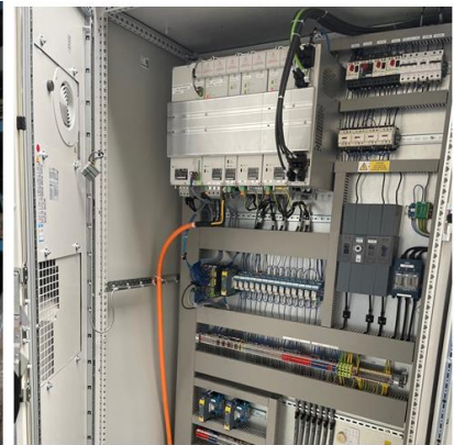
Cabinet components
